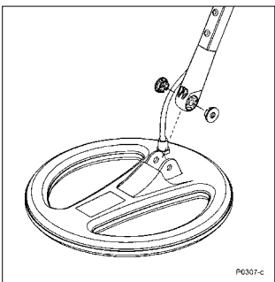
Figure 2.2 Inserting coil yoke into bracket
