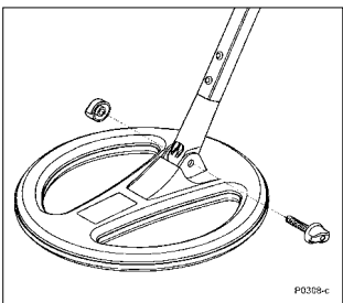
Figure 2.3 Securing yoke to search coil
