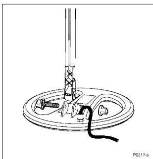
Figure 2.18 Removing yoke from search coil
