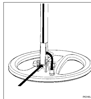
Figure 2.15 Prizing off coil yoke cover
