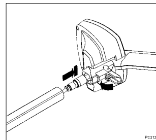
Figure 2.8 Inserting shaft assembly into control box
