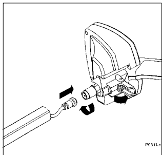
Figure 2.6 Attaching coil cable to control box
