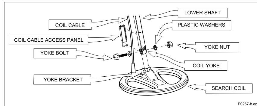
Figure 2.14 Replacing the search coil
