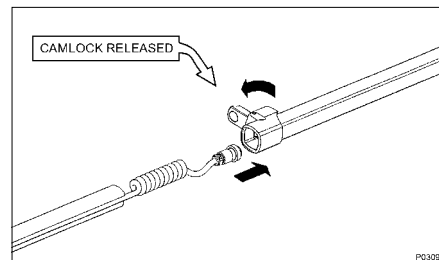
Figure 2.4 Feeding coil cable into upper shaft
