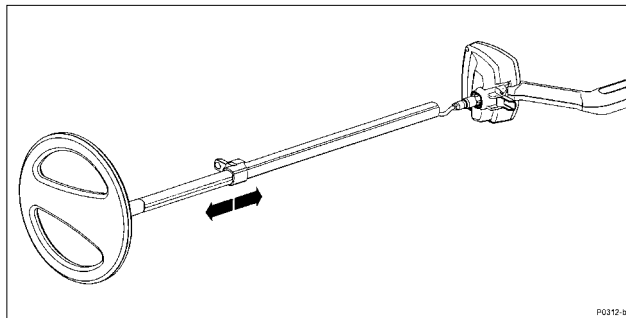
Figure 2.7 Preventing the coil cable 'bunching'
